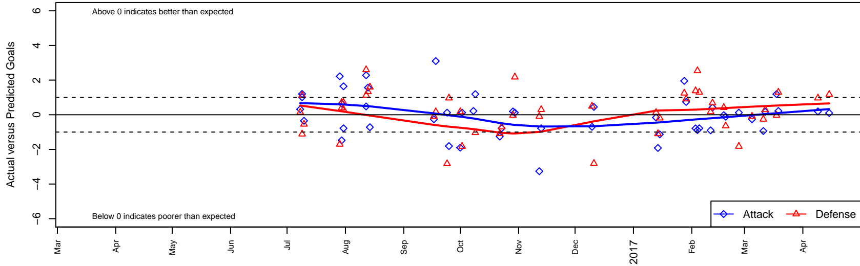
HSC GPS Oregon G02 Dots are actual minus expected GF (blue circles) and GA (red triangles). Blue line is smoothed change in attack strength. Red is smoothed change in defense strength.
